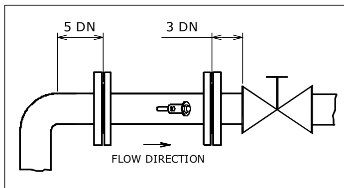
Fig. 7 - Minimum straight piping section before closing valve
