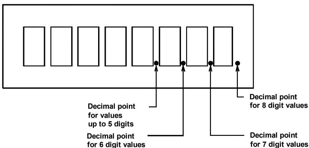
Fig. 15 - Decimal point positions on the display
