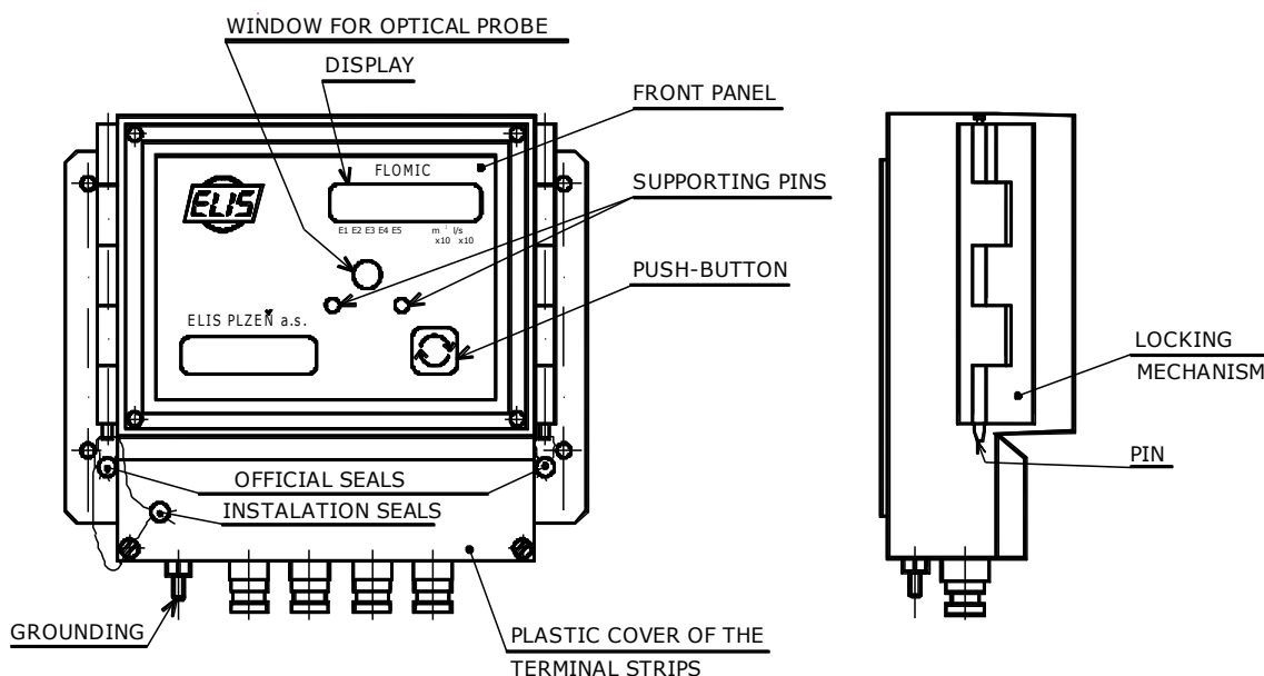
Fig. 4 - Transmitter - description
