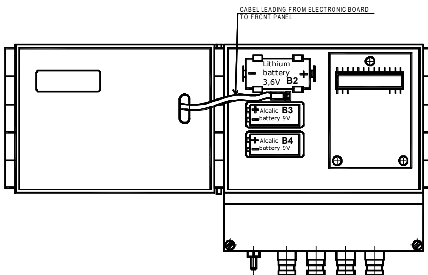
Fig. 20 - Battery replacement
