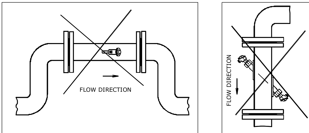
Fig. 11 - Examples of incorrect sensor placement
