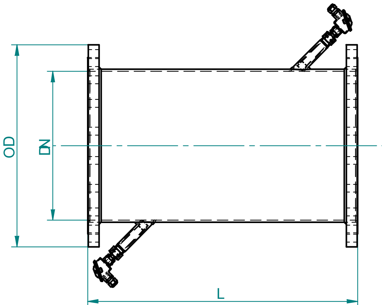
Fig. 1 - Dimensional sketch of meter sensor
