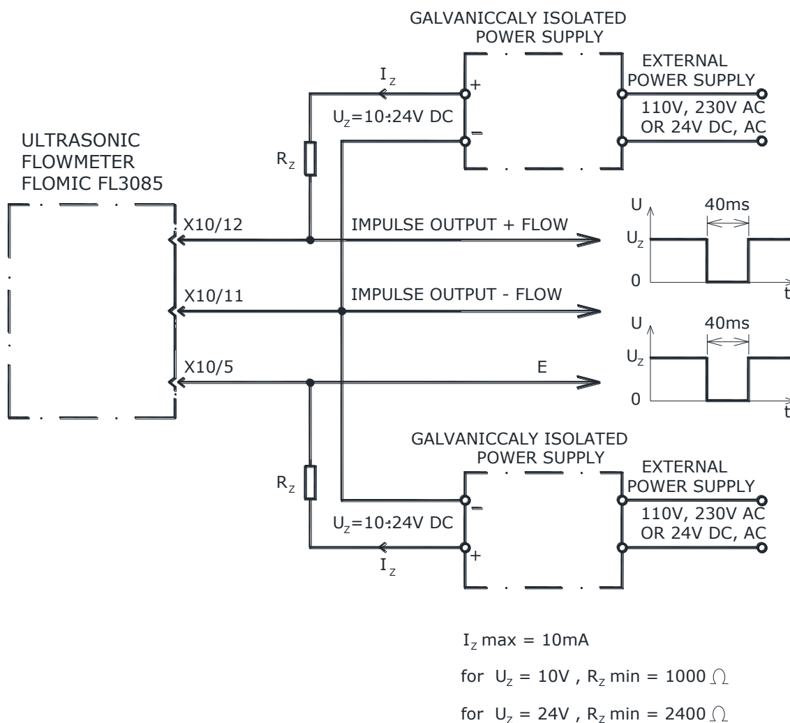
Fig 14 a) Connection of pulse output to an external power source
