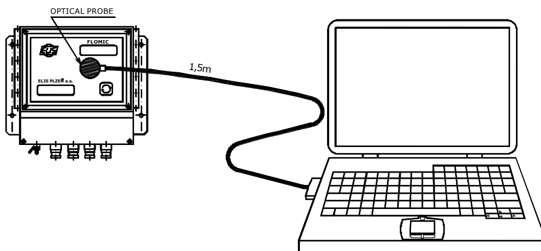
Fig. 17 - Communication via optical cable
