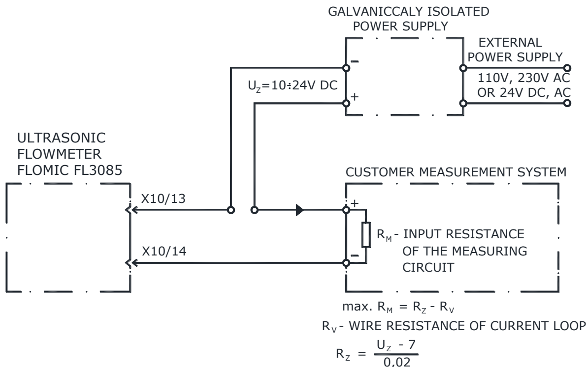
Fig. 14 b) Connection of current output to an external power source
