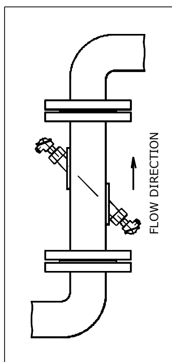
Fig. 10 - Sensor located in vertical piping section
