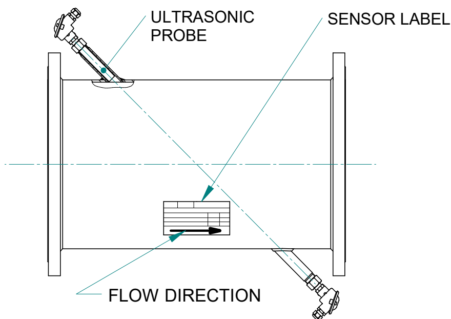
Fig. 3 - Ultrasonic probe assembly
