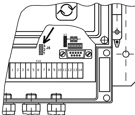
Fig. 16 - Change in the pulse length setting
