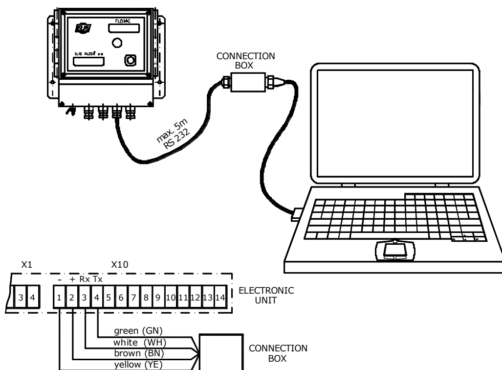
Fig. 18 - Communication via RS-232 line
