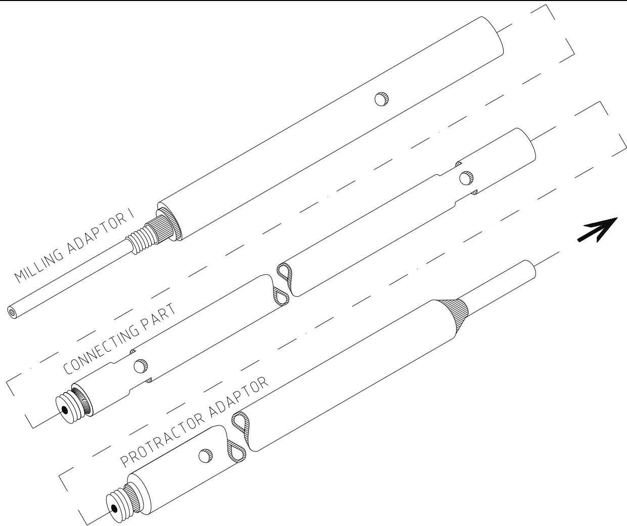
Fig. 25 - Rectification pin assembly parts
