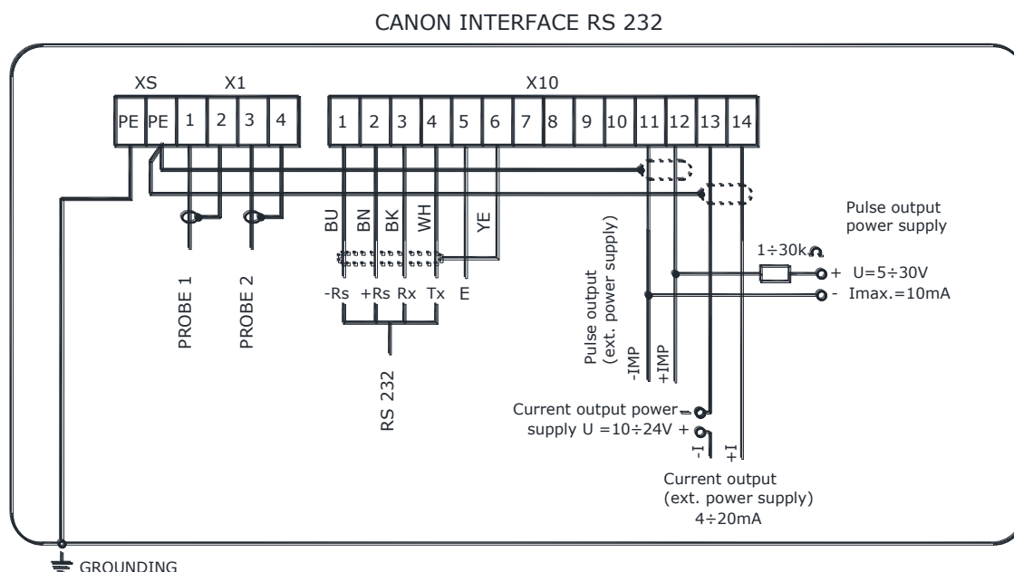
Fig. 30 - Input and output signal connections of the UP 8.00 electronic unit
