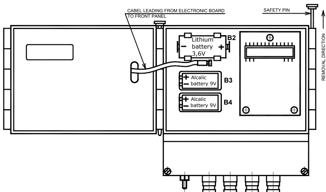
Fig. 45 - Battery replacement
