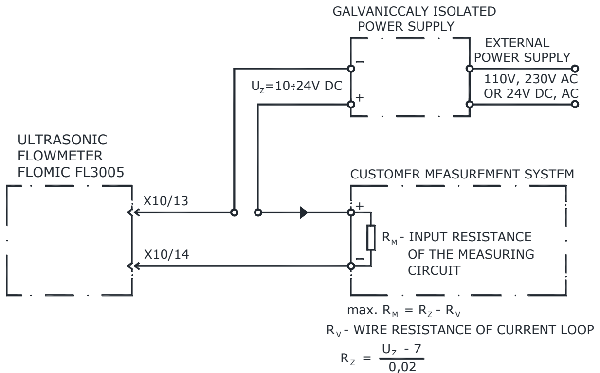
Fig 41 Connection of current output to an external power source
