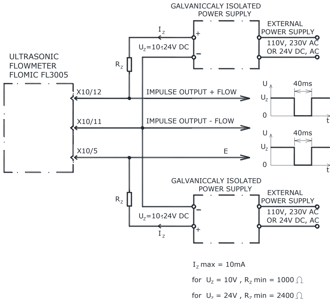
Fig 40 Connection of pulse output to an external power source
