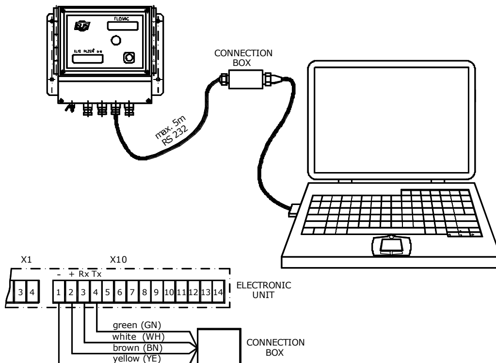
Fig. 44 - Communication via RS 232 interface
