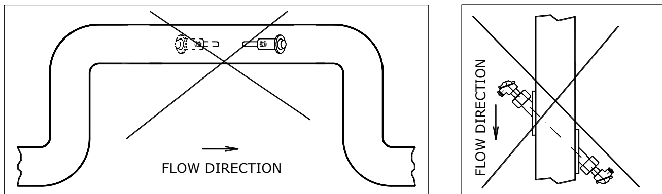
Fig. 18 - Examples of incorrect sensor placement
