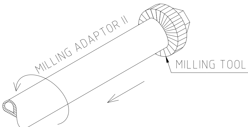
Fig. 27 - Facing of the seating surface on the inaccessible welded-on piece
