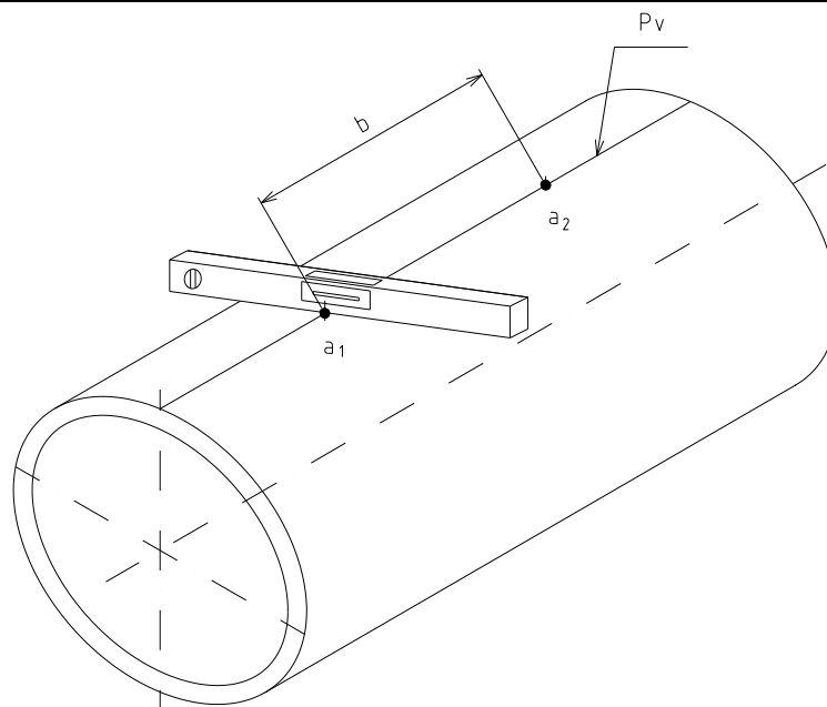
Fig. 21 - Top surface line marking on meter piping
