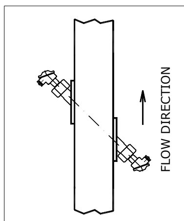
Fig. 17 - Sensor fitted into a vertical piping section
