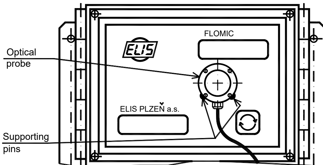
Fig. 42 - Working position of the optical probe
