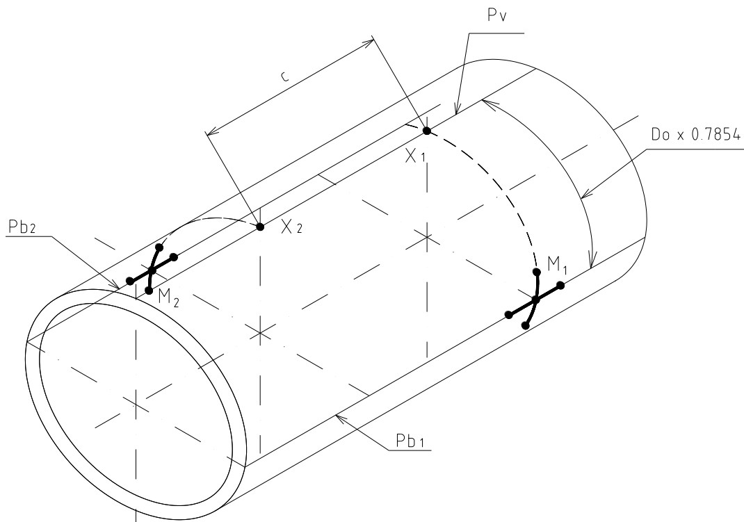
Fig. 22 - Laying out of key installation points
