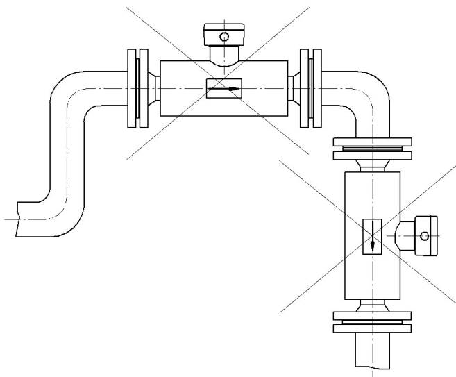
Examples of incorrect sensor placement
