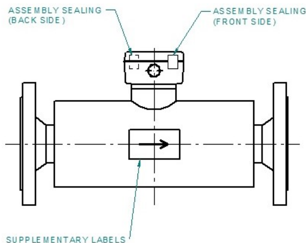
Sealing of sensor UC3.0
