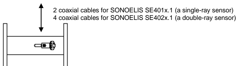
Sensor UC 7.0 (a single-ray) / UC 7.2 (a double-ray)
